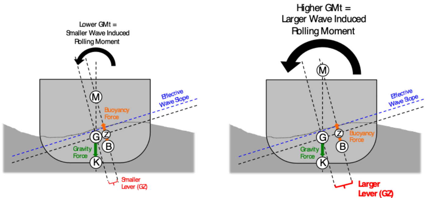
Figure 4 – Induced Wave Torque Lever with Higher GM T
