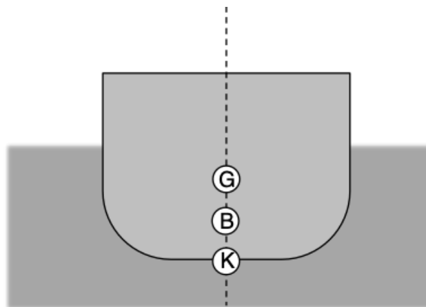
Figure 1 – Hull at Zero Heel Angle
